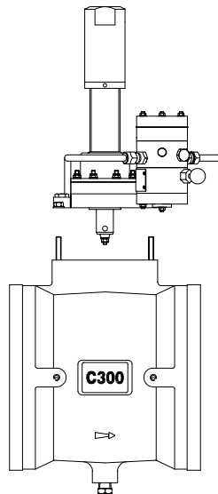
Regulating with Actuator DV050 1007
